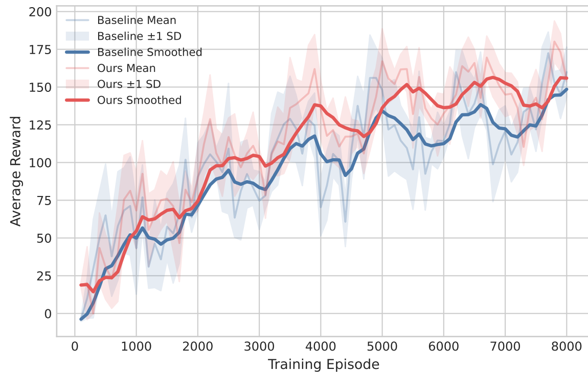
Highway Dense: Baseline vs. Ours (5 Seeds)
