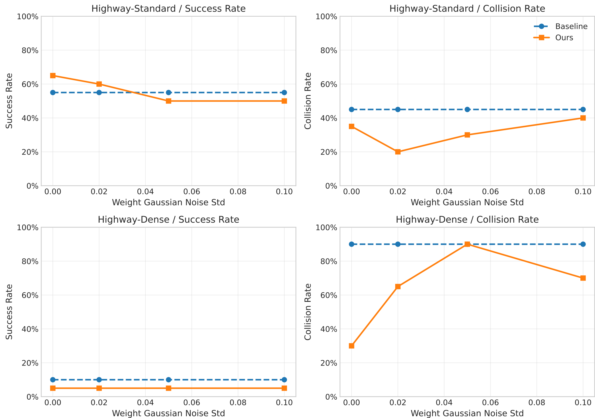
Figure 5. Weight Noise Robustness
