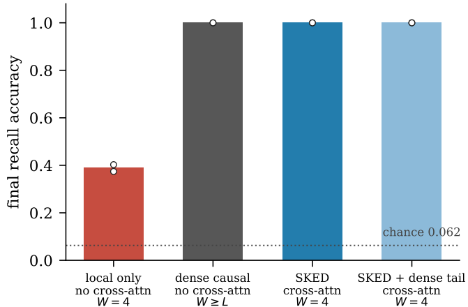
(a) final accuracy, 2 seeds
