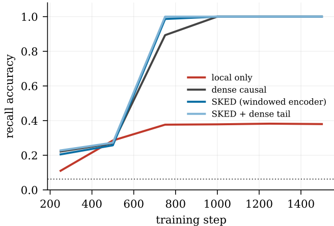
(b) learning curves, mean of 2 seeds
