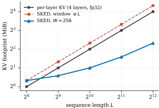
(a) measured prototype (4 layers, CPU)
