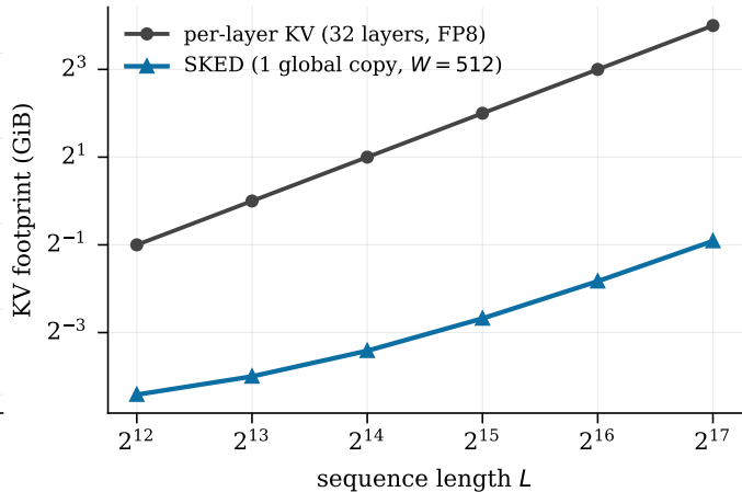
(b) analytic, spec config (not measured)
