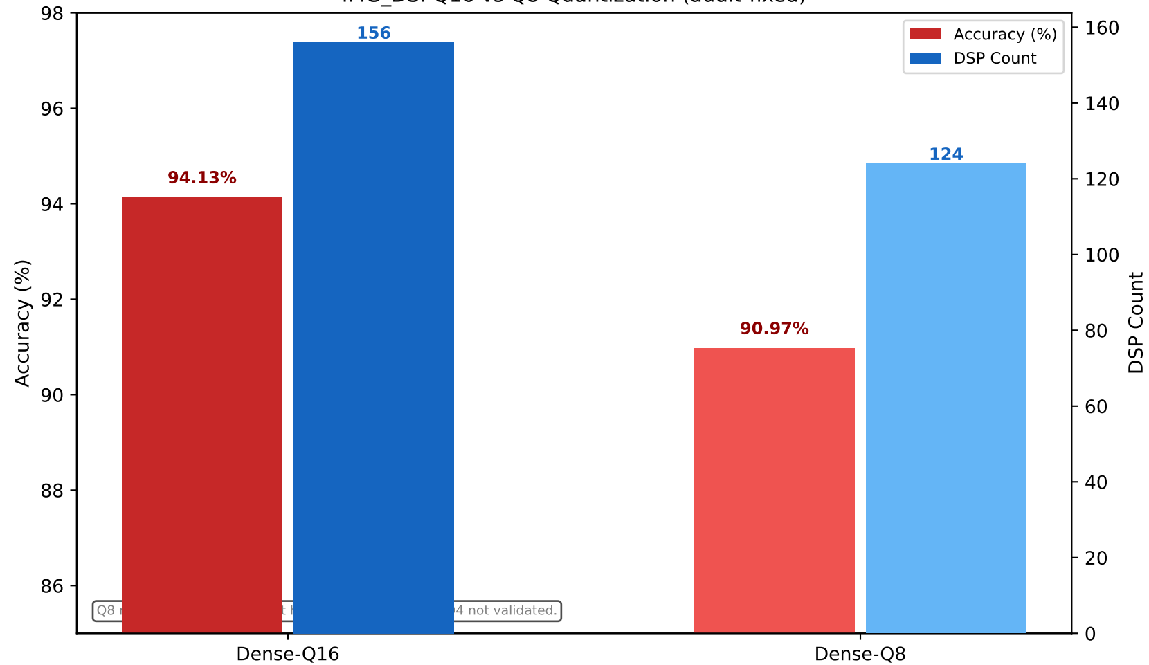
IMG_DS: Q16 vs Q8 Quantization (audit-fixed)
