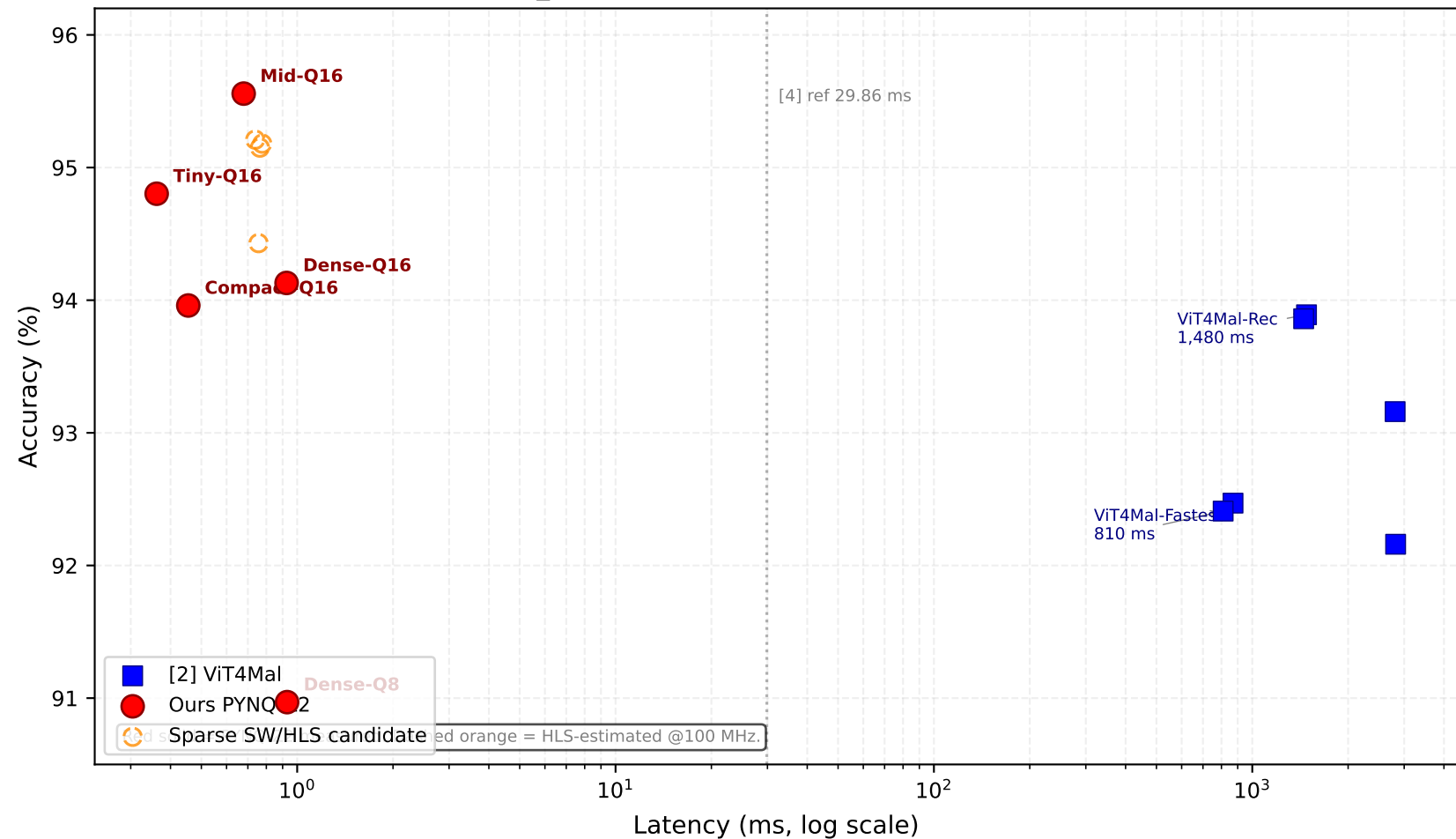
IMG_DS Pareto Frontier: Accuracy vs Latency
