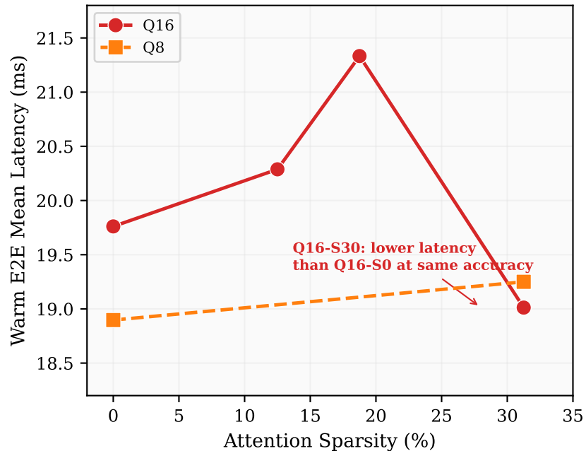
(b) Warm E2E Latency vs Sparsity
