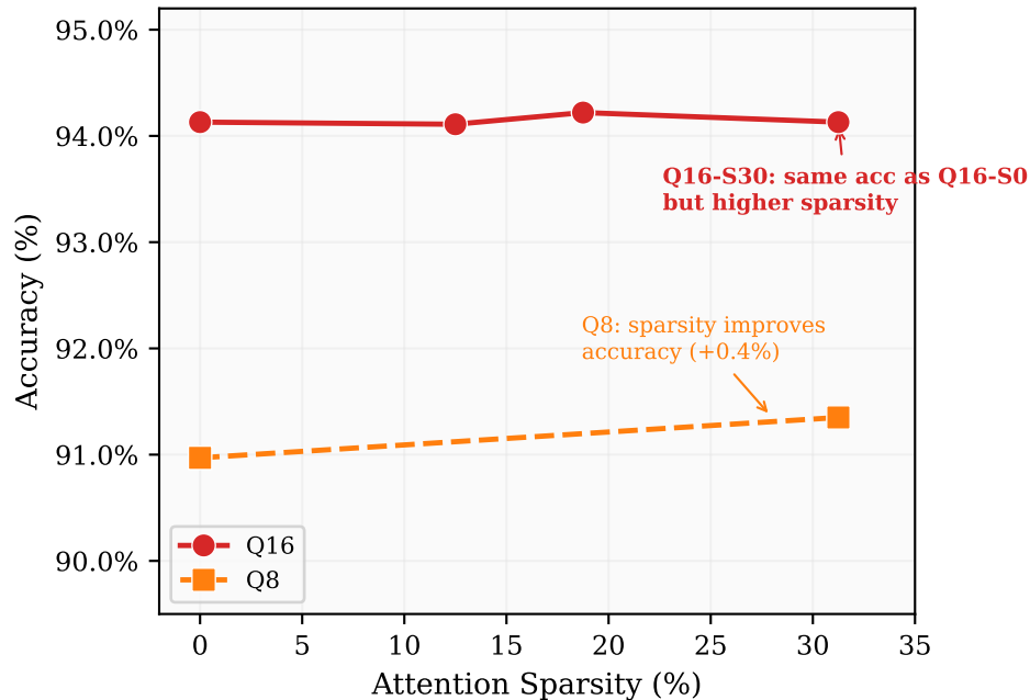
(a) Accuracy vs Sparsity
