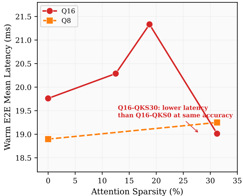
(b) Warm E2E Latency vs Sparsity
