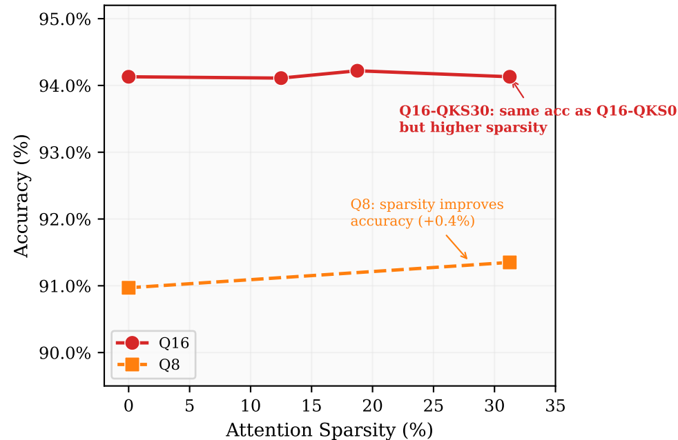
(a) Accuracy vs Sparsity
