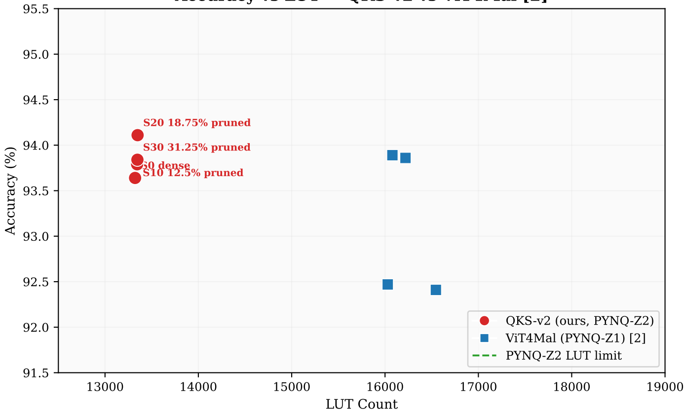
Accuracy vs LUT — QKS-v2 vs ViT4Mal [2]
