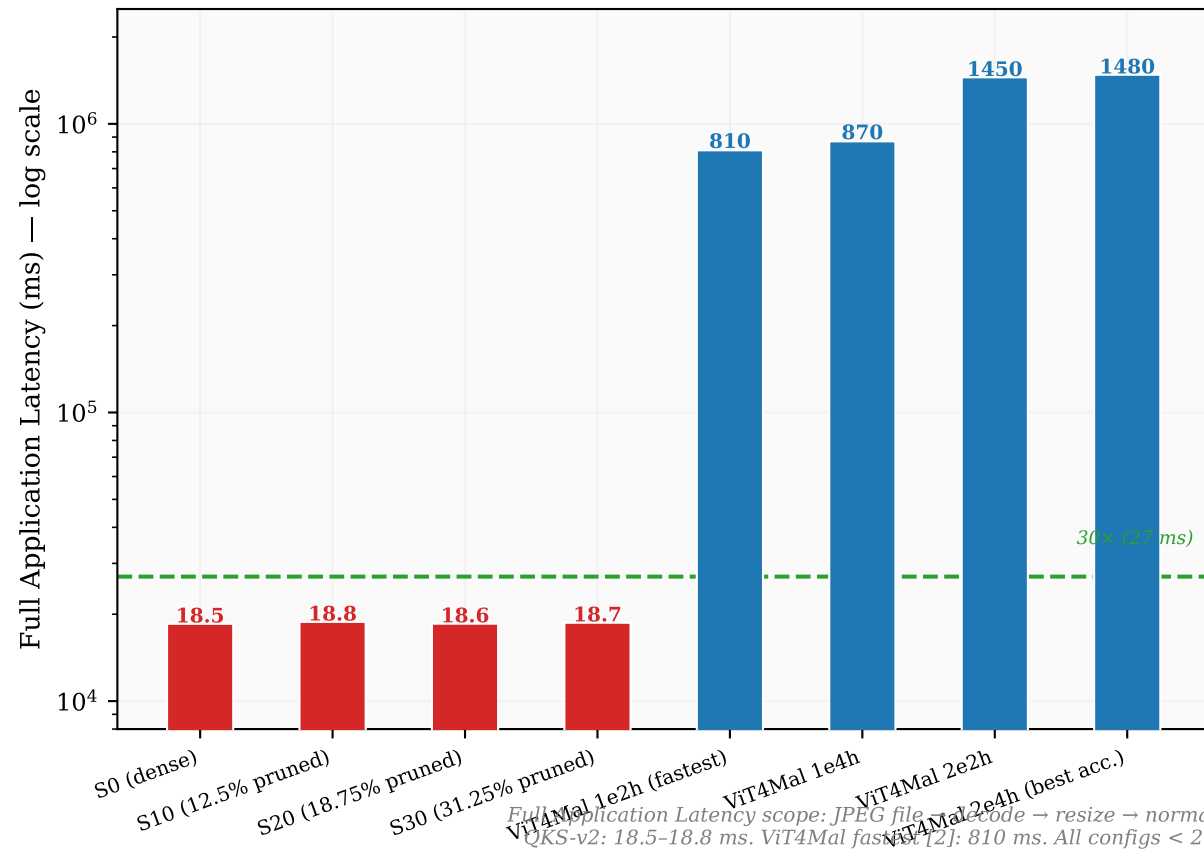
(a) Full Application Latency (same scope as ViT4Mal [2] Table 13)
