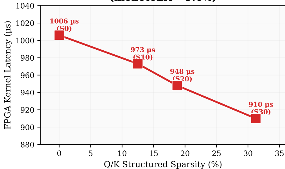
(a) FPGA Kernel Latency vs Sparsity (monotonic -9.6\% )
