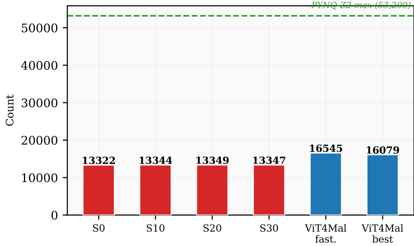
Flip-Flops
