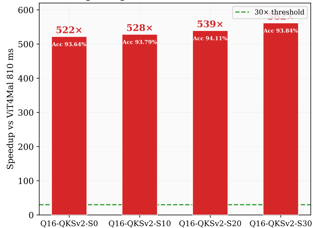
(b) Speedup vs ViT4Mal Fastest (810 ms)
