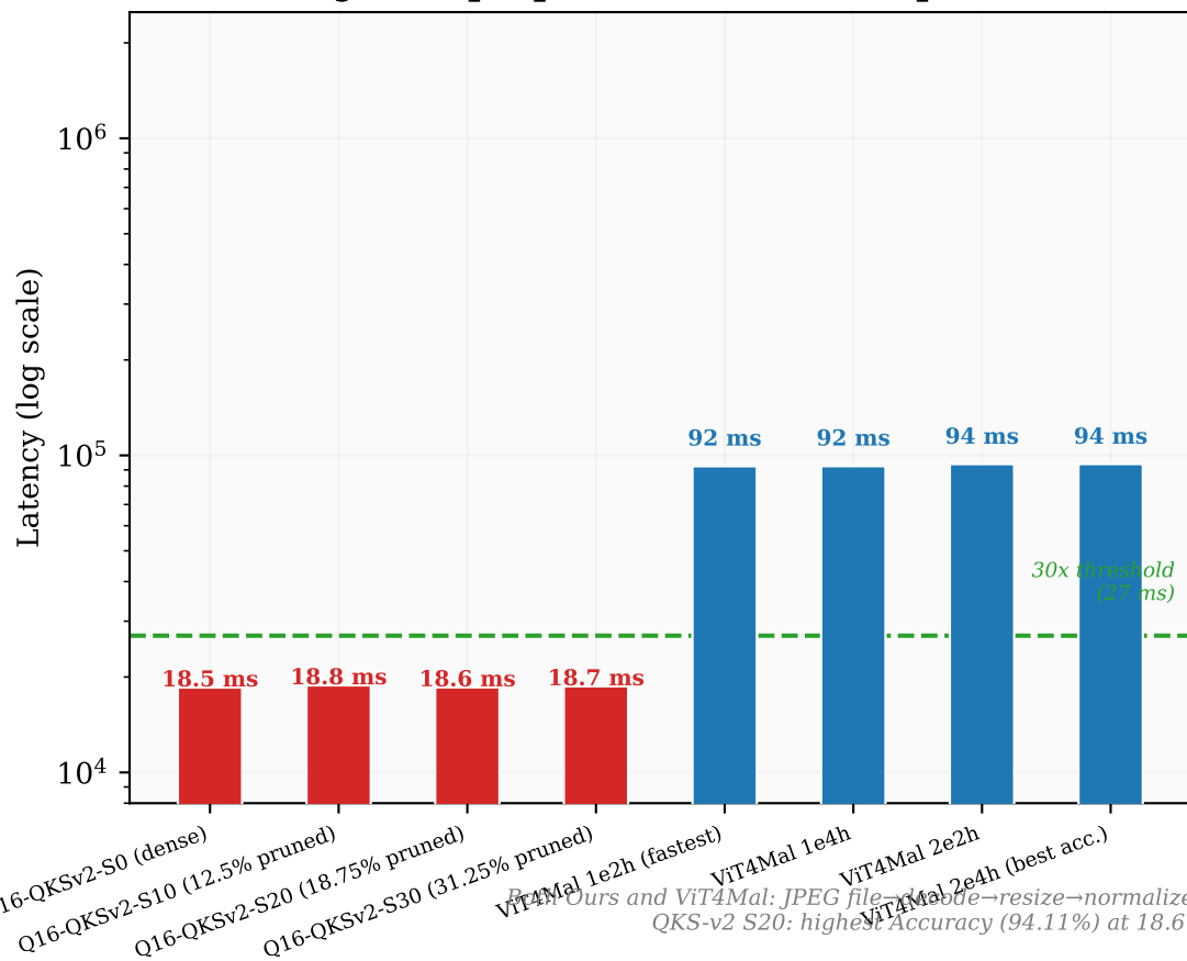
(a) Full Application Latency (JPEG→preprocess→FPGA→output)
