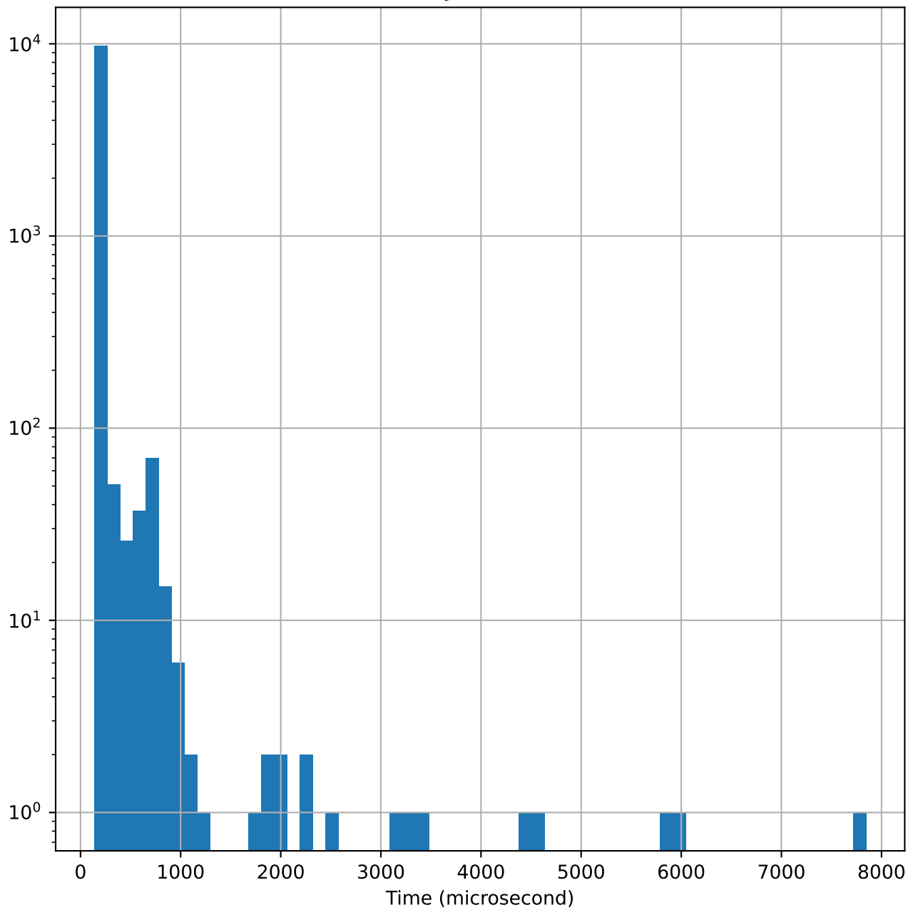
Latency distribution
