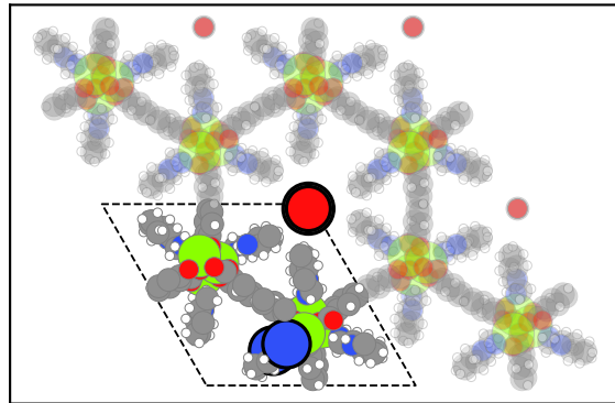
(c) MOF + CO 2 (in pore)
