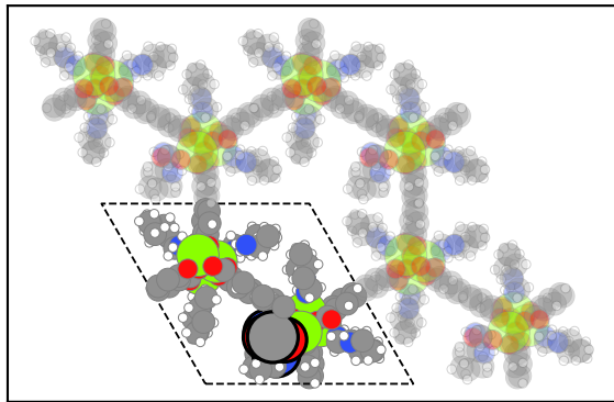
(b) MOF + CO 2 (carbamate)
