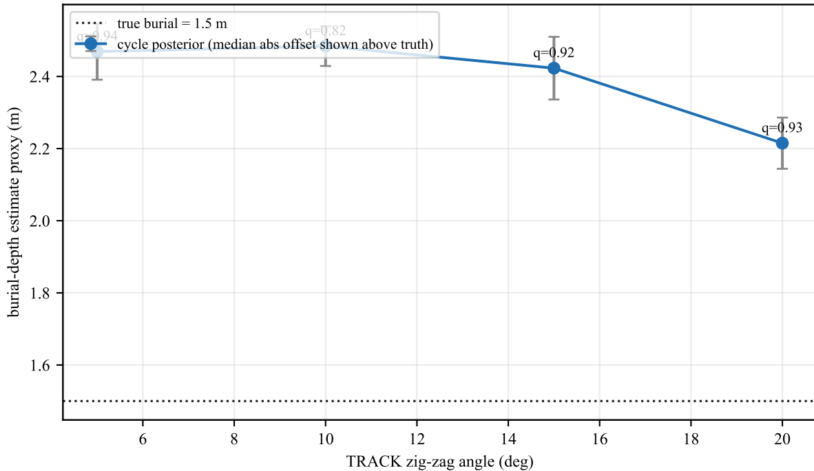
Illustrative cycle-local burial posterior (1.5 m depth)
