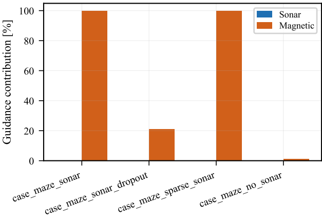
Sonar / magnetic contribution
