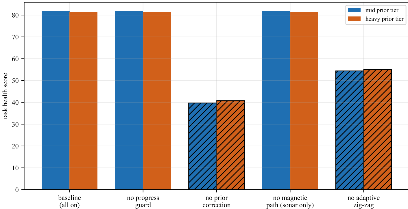
B3: leave-one-out ablation (hatched = task failed)
