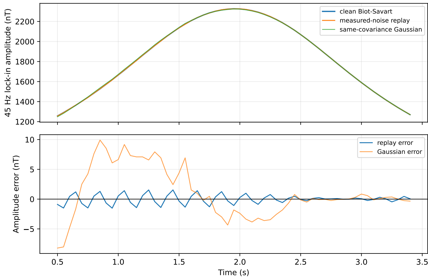
Noise-injected Biot-Savart replay: 1780675809_291477.npz
