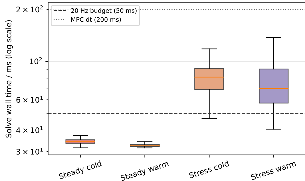
Target-platform MPC latency
