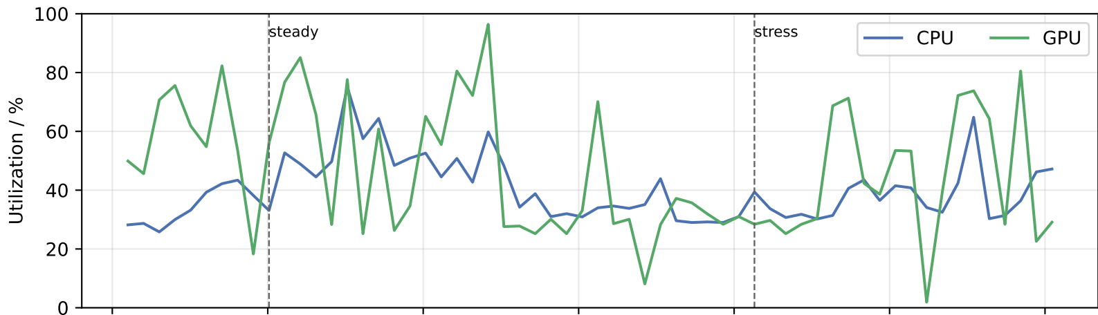
Jetson resource profile during clean MPC microbenchmark
