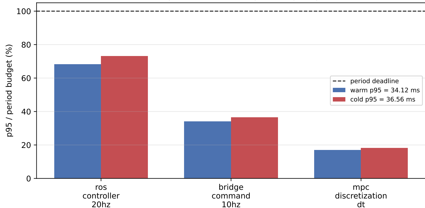
Steady-state solver budget occupancy
