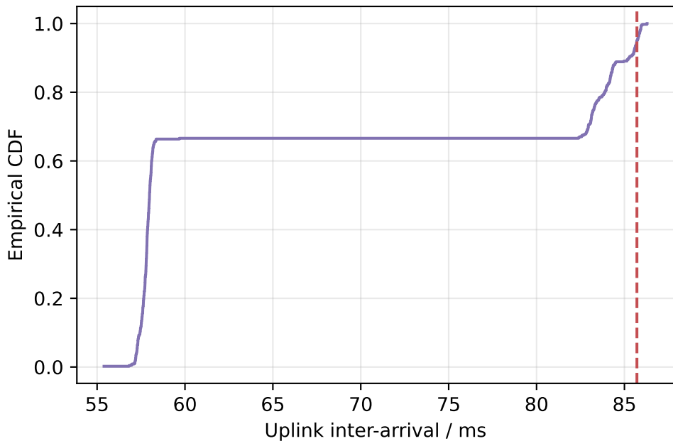
Empirical distribution
