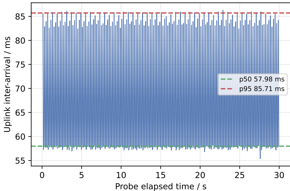
Arrival-interval timeline
