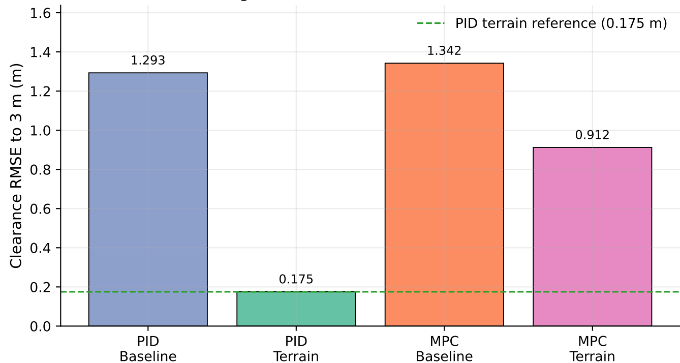
Terrain-Following Clearance Error: PID/MPC x Baseline/Terrain
