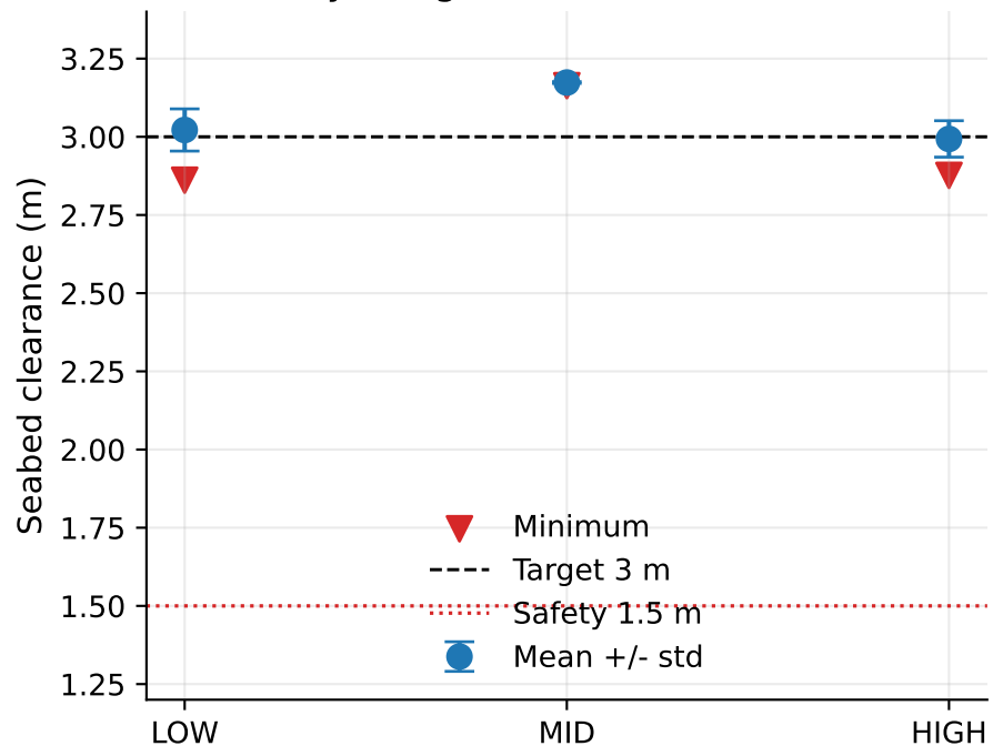
Safety Margin Across Terrain Levels
