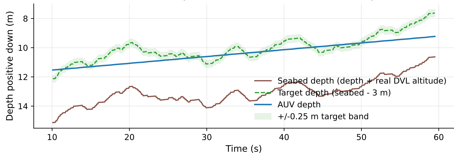
MPC Terrain (clearance source: real DVL altitude)
