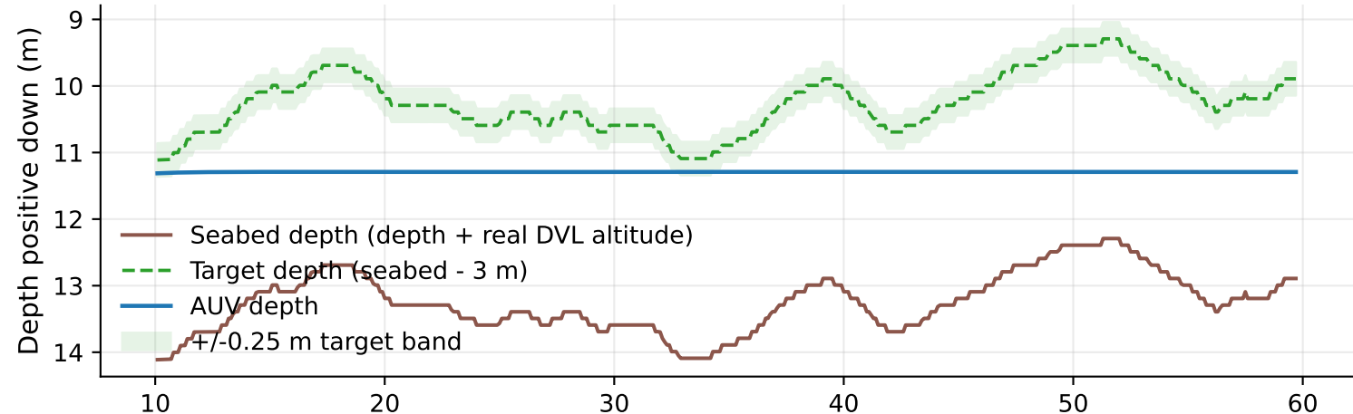
MPC Terrain (clearance source: real DVL altitude)
