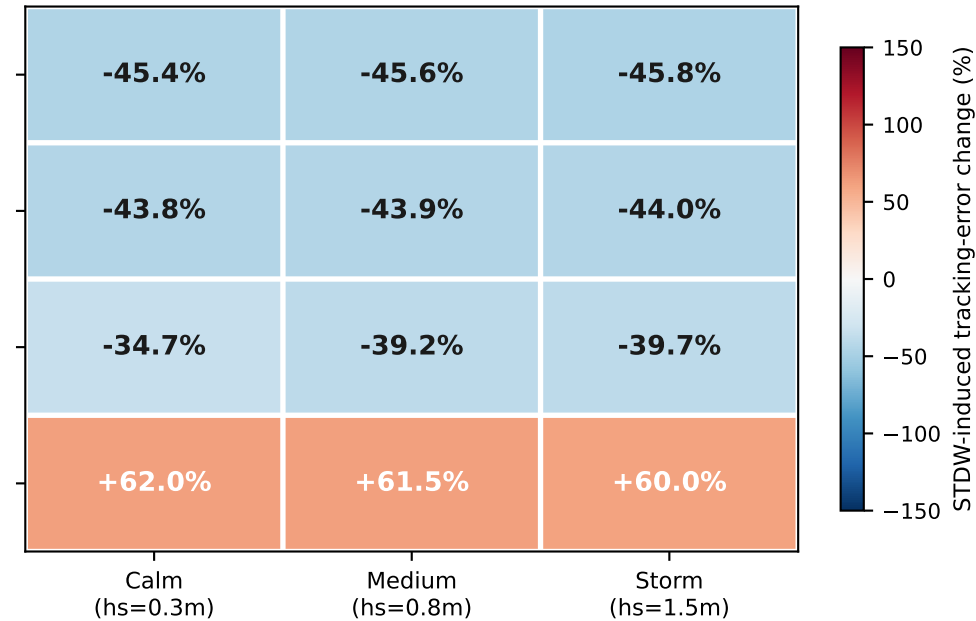
Post-drift tail error change (5s-RMS filtered)
