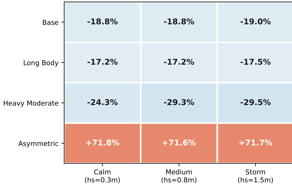
Full-trajectory tracking-MSE change
