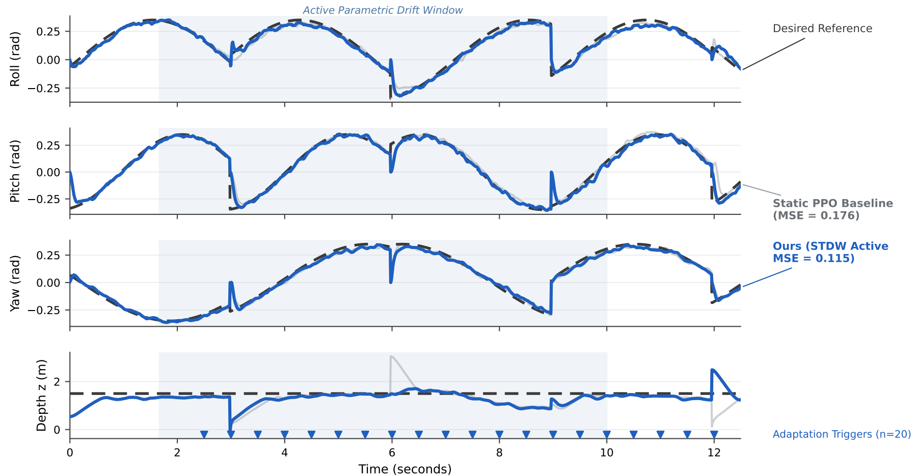
Attitude-depth tracking overlay under Storm sea state + COM drift (Heavy hull)
