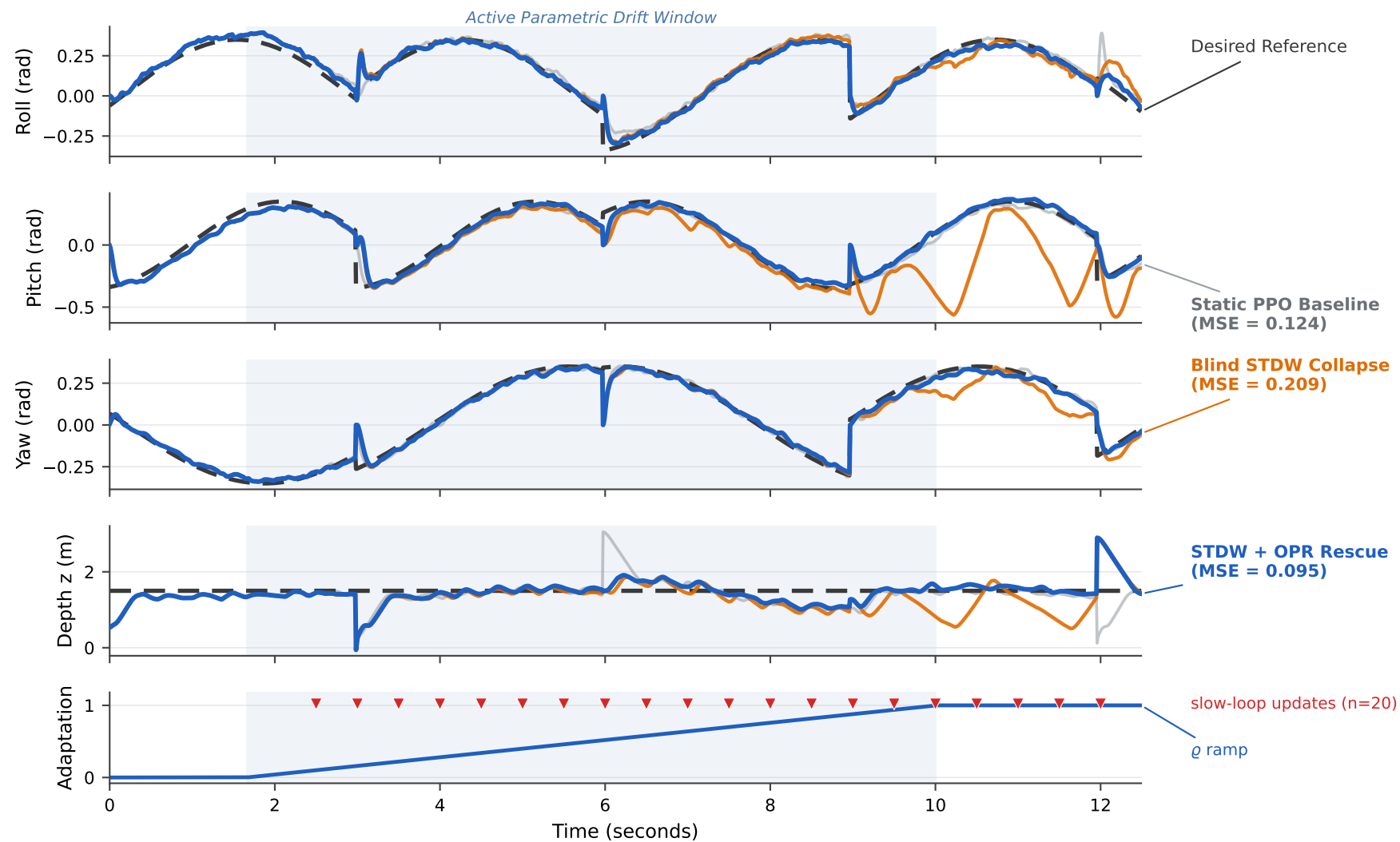
OPR rescues the Asymmetric hull from blind-STDW collapse (Storm sea state, shared reference)
