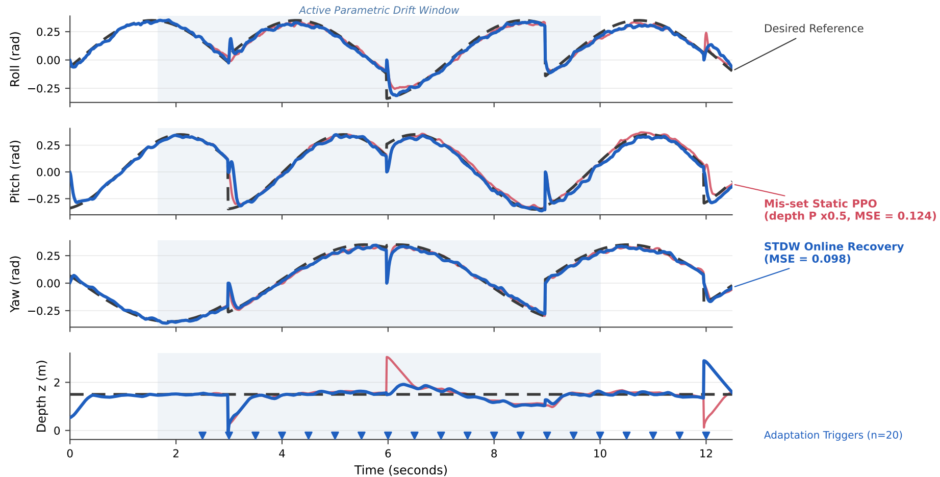
STDW recovers a mis-set initial controller online (depth P gain x0.5, Base hull, storm sea state)
