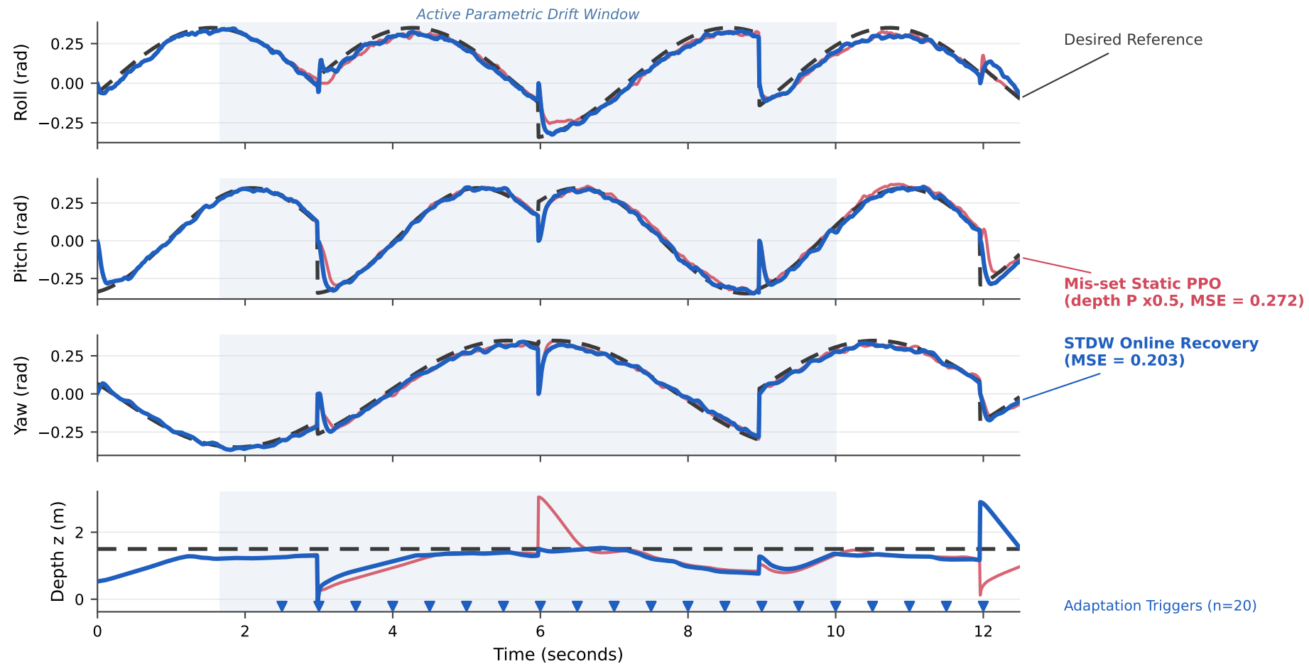
STDW recovers a mis-set initial controller online (depth P gain x0.5, Heavy hull, storm sea state)
