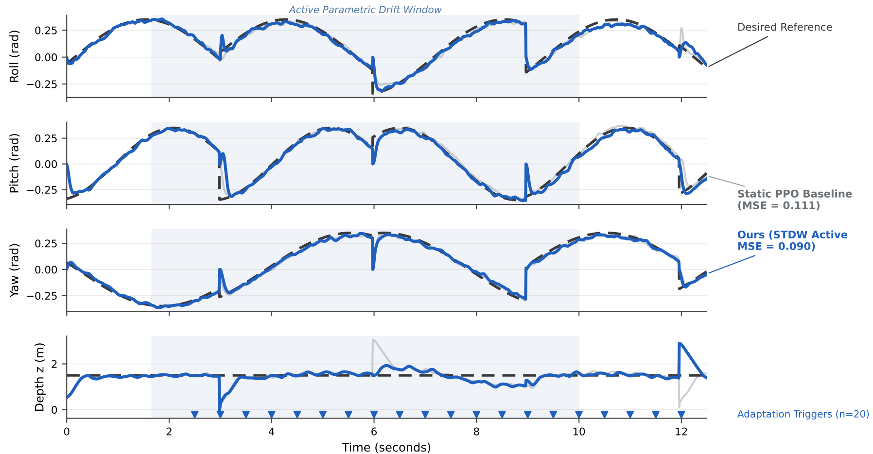
Attitude-depth tracking overlay under Storm sea state + COM drift (Base hull)
