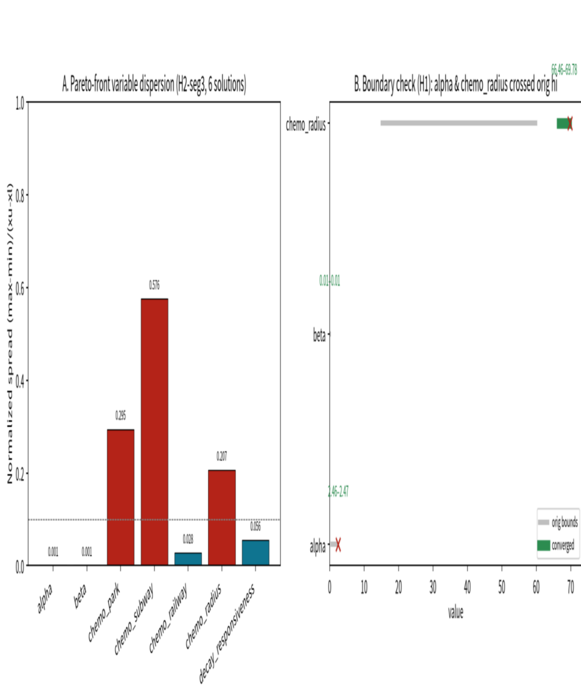
Parameter sensitivity – Bio-Physarum + NSGA-II (real runs, method validation)
