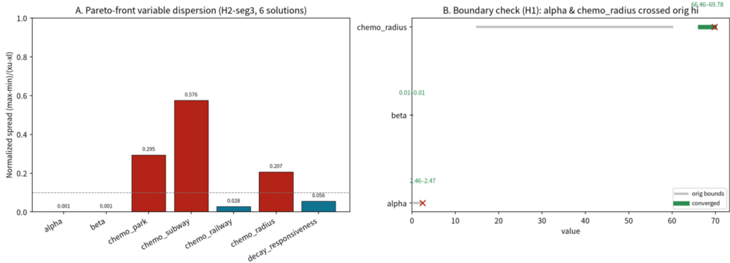
Parameter sensitivity — Bio-Physarum + NSGA-II (real runs, method validation)
