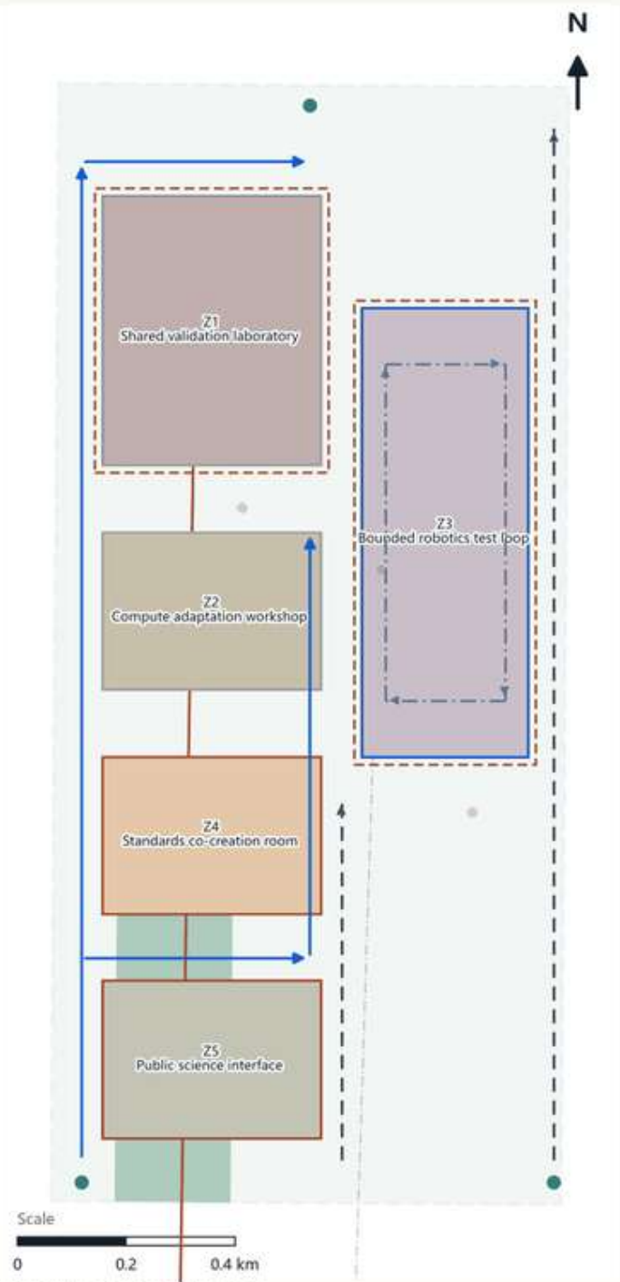
Conceptual indicative dimensions; pending survey and professional verification Source: official package geometry/*geojson and metrics.json (recomputed in EPSG:4548)
