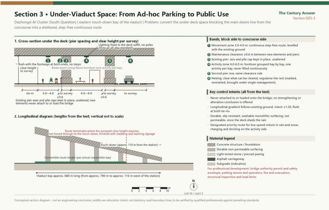
Section DZS-3: under-bridge space from ad-hoc parking to public use (conceptual section, no engineering conclusions)
