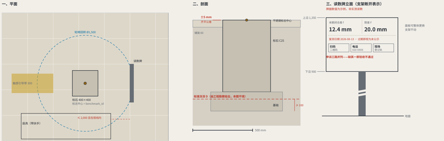
FIG.16 The benchmark and its reading plate, as a construction detail
