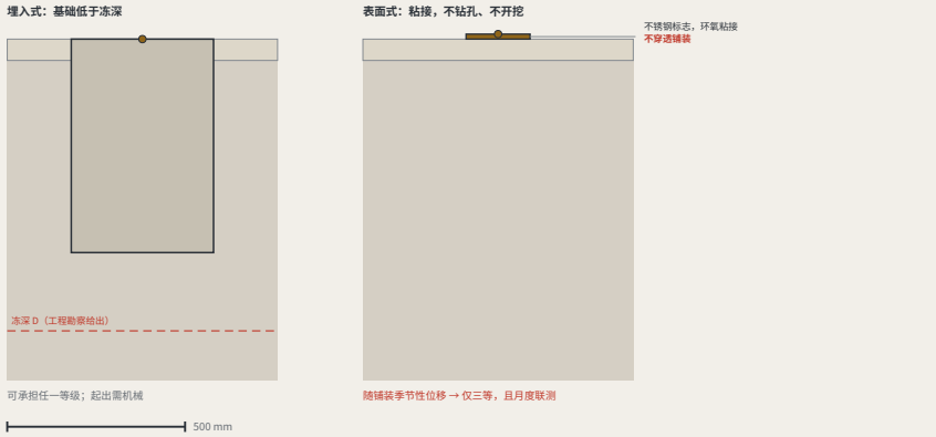
FIG.19 Monuments beside heritage fabric: the no-drilling construction and its setback rule 类型图，不表示朝向
