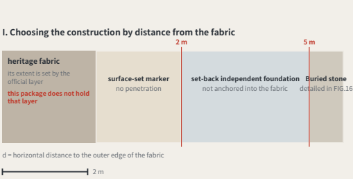
Monuments beside heritage fabric: the no-drilling construction and its setback rule
