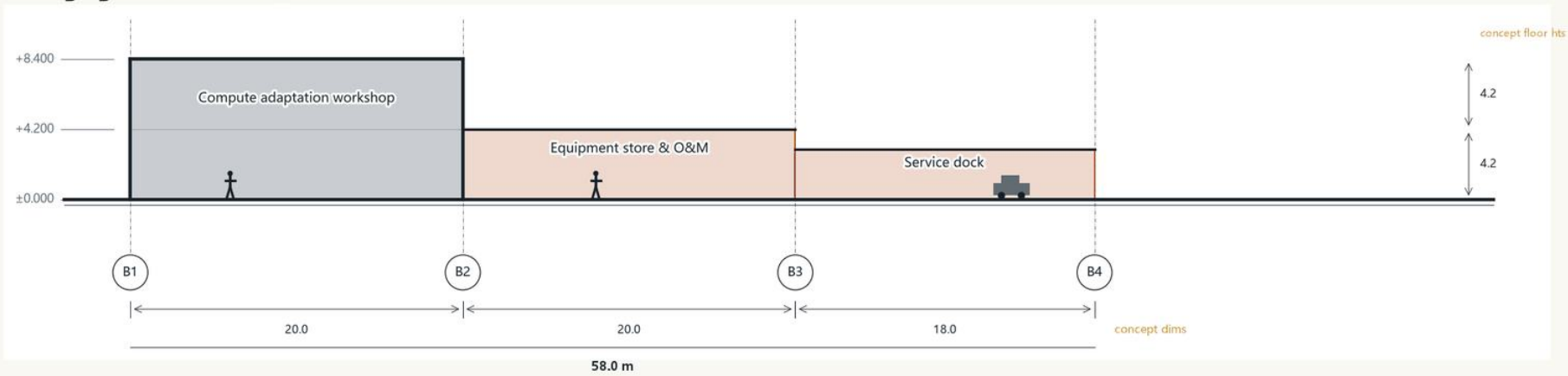
Secondary section: workshop • logistics • service dock
