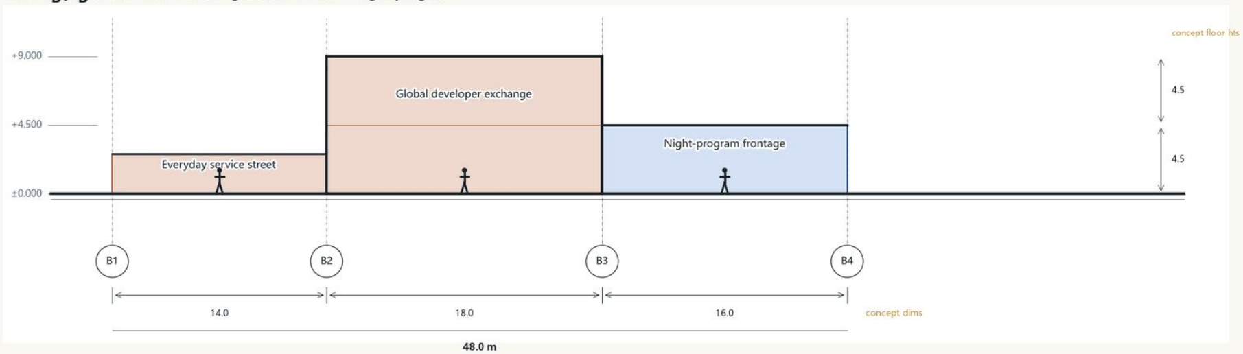
Secondary section: service street • global-node wall • night program
