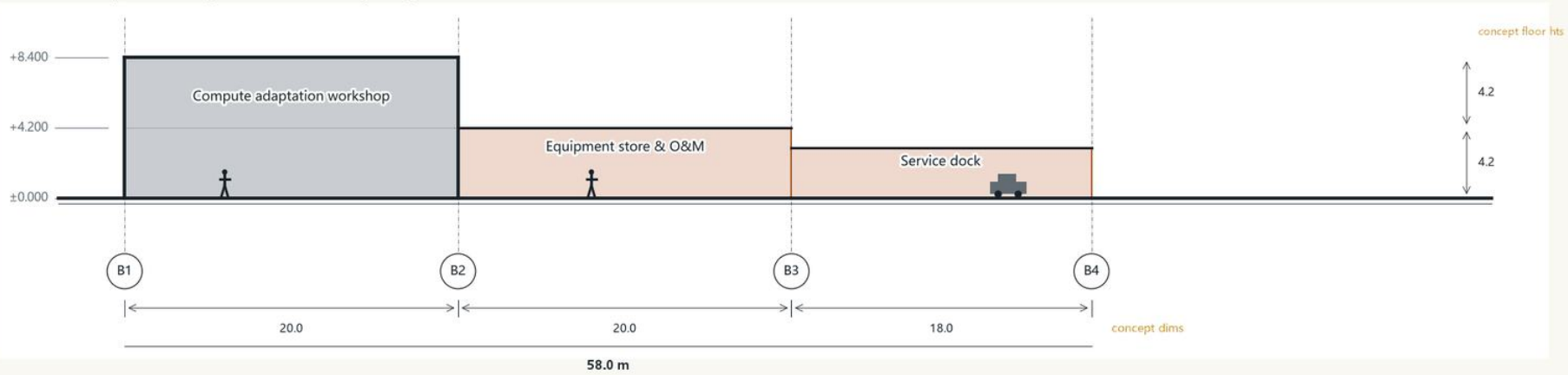
B—B' | Secondary section: workshop • logistics • service dock
