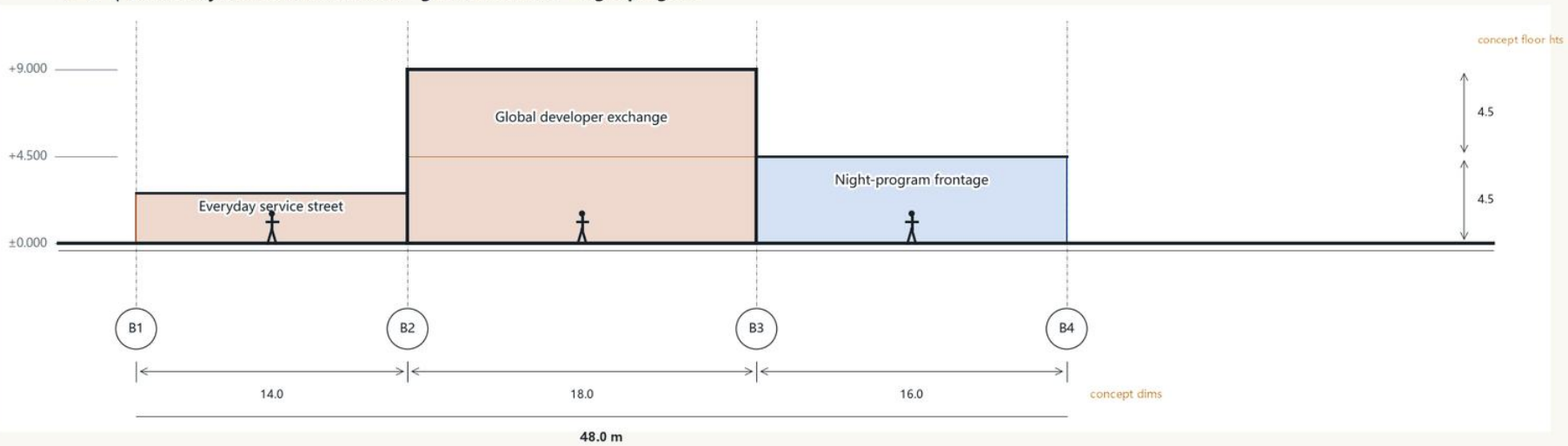
B—B' | Secondary section: service street • global-node wall • night program
