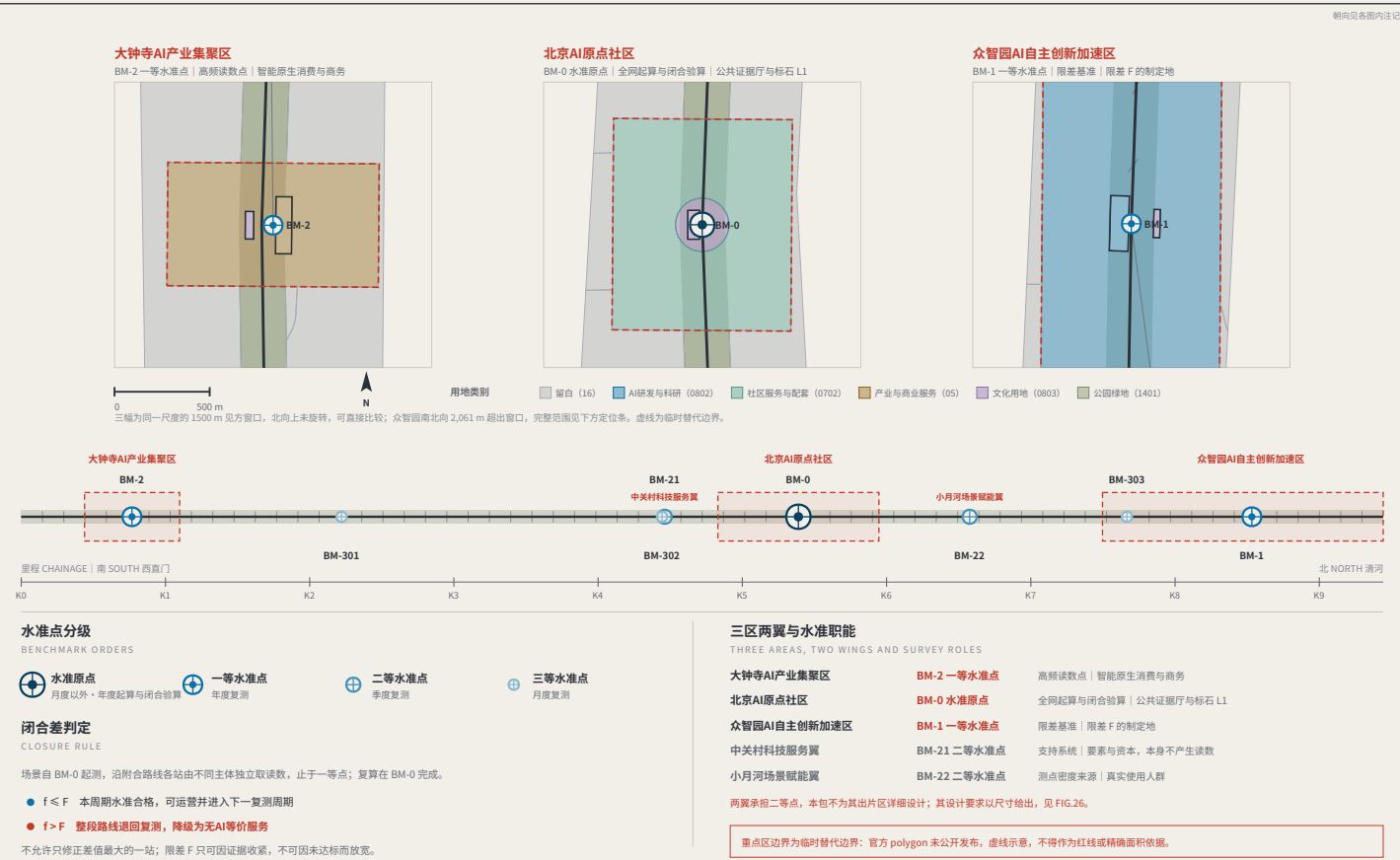
FIG.04 THREE AREAS, TWO WINGS AND BENCHMARK LAYOUT
