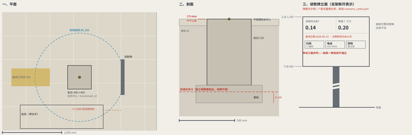
FIG.16 The benchmark and its reading plate, as a construction detail
