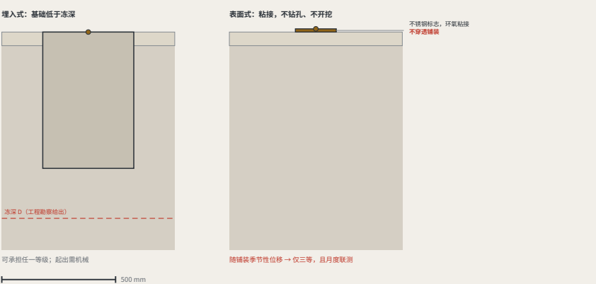
FIG.19 Monuments beside heritage fabric: the no-drilling construction and its setback rule
