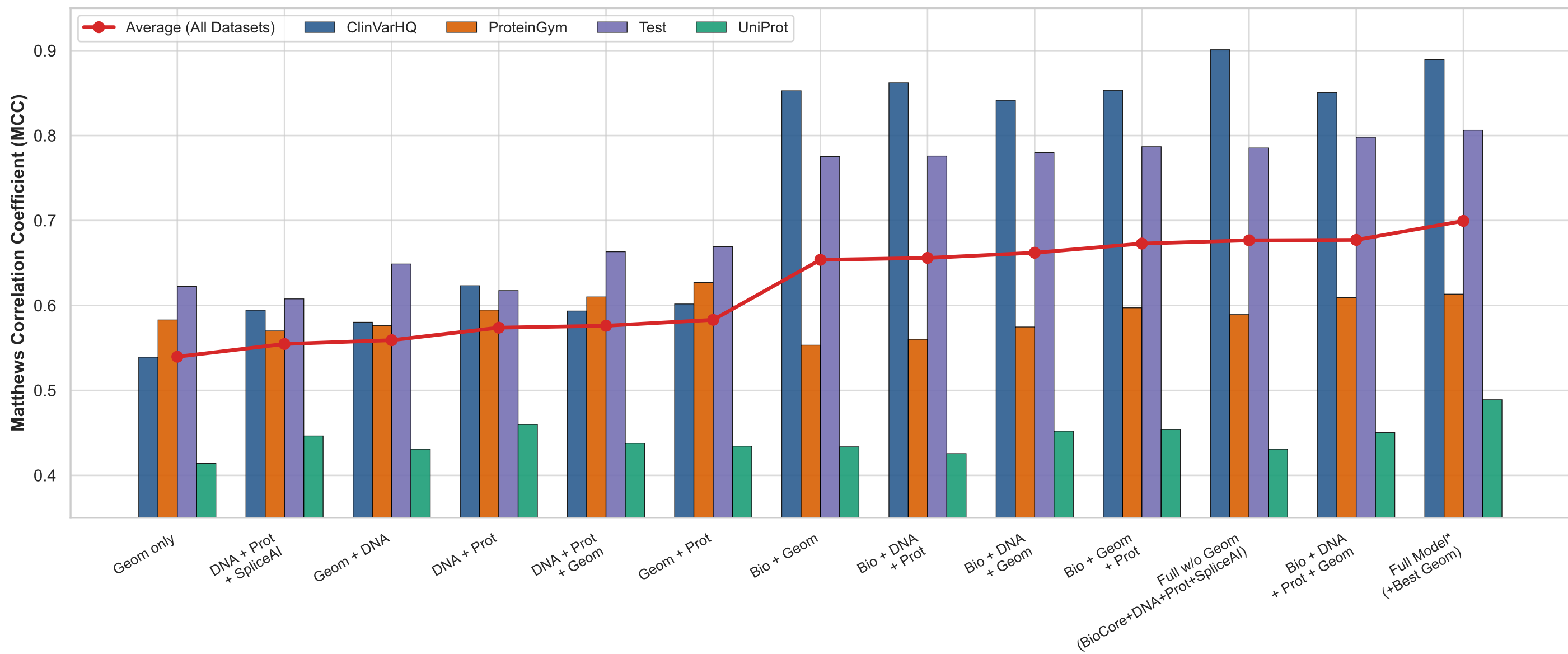
(A) Comprehensive Modality Ablation (mean pooling, nt_v2_500m, esm1b_650m, Pure_XGBoost_Concat)
