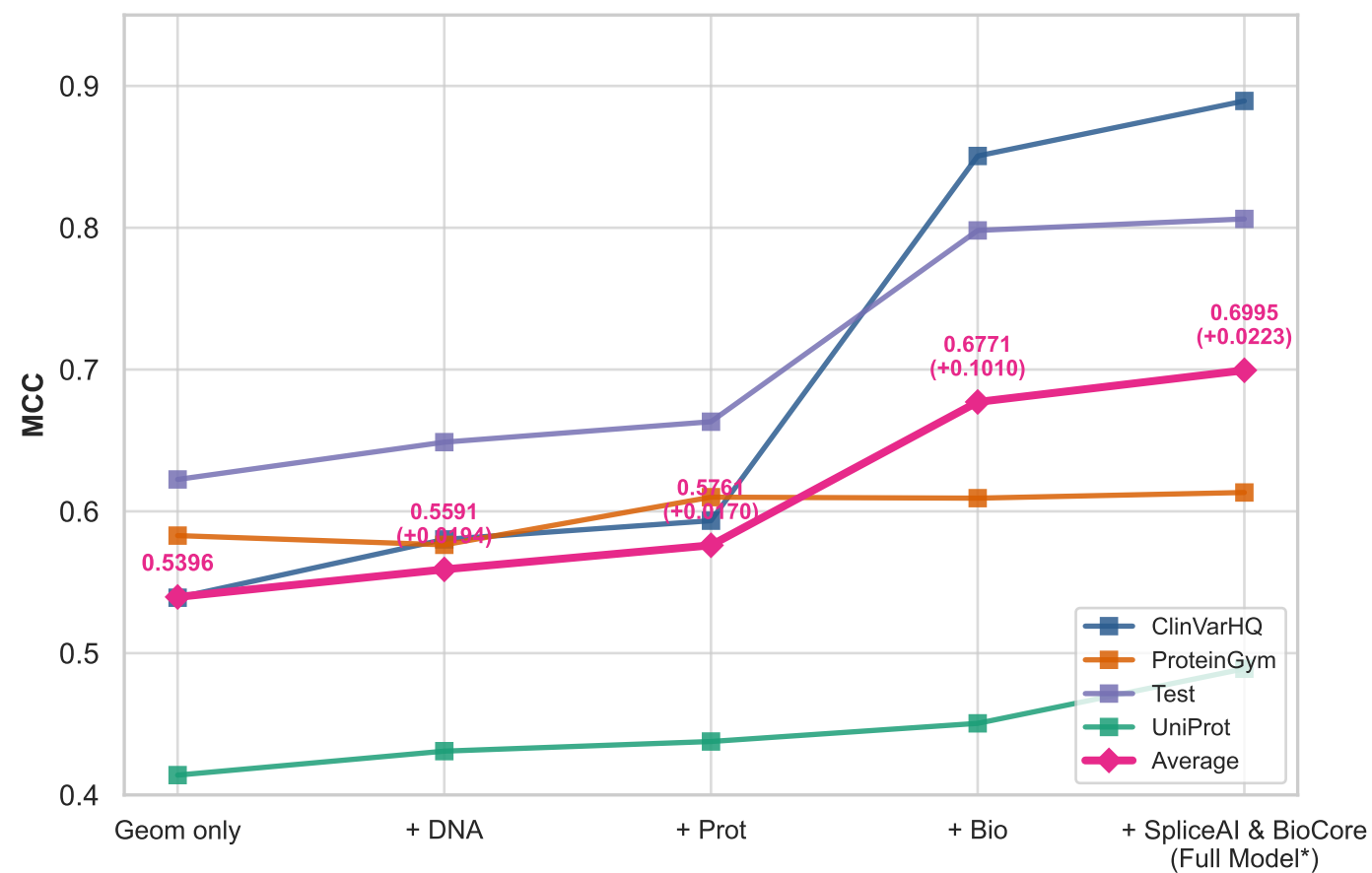
(B) Cumulative Modality Addition (Progression)
