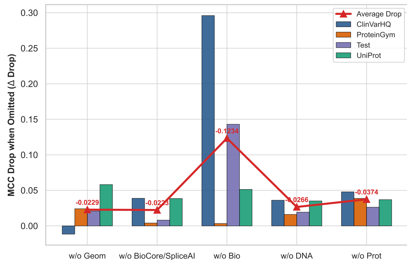
(C) Leave-One-Out Impact (Drop Relative to Full Model)
