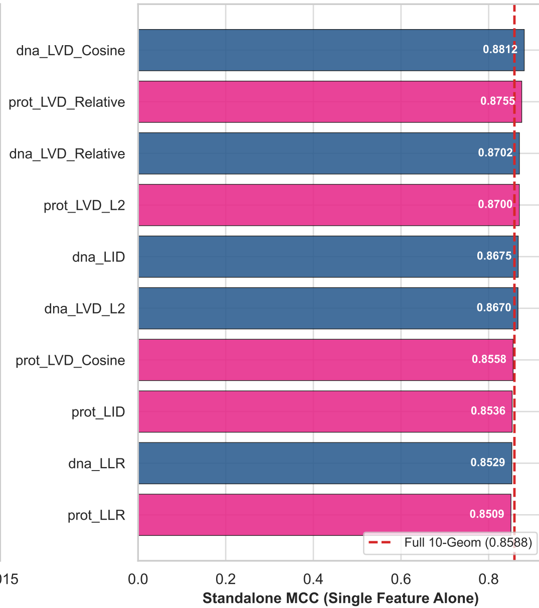
(B) Standalone Feature Performance (ClinVarHQ Benchmark)
