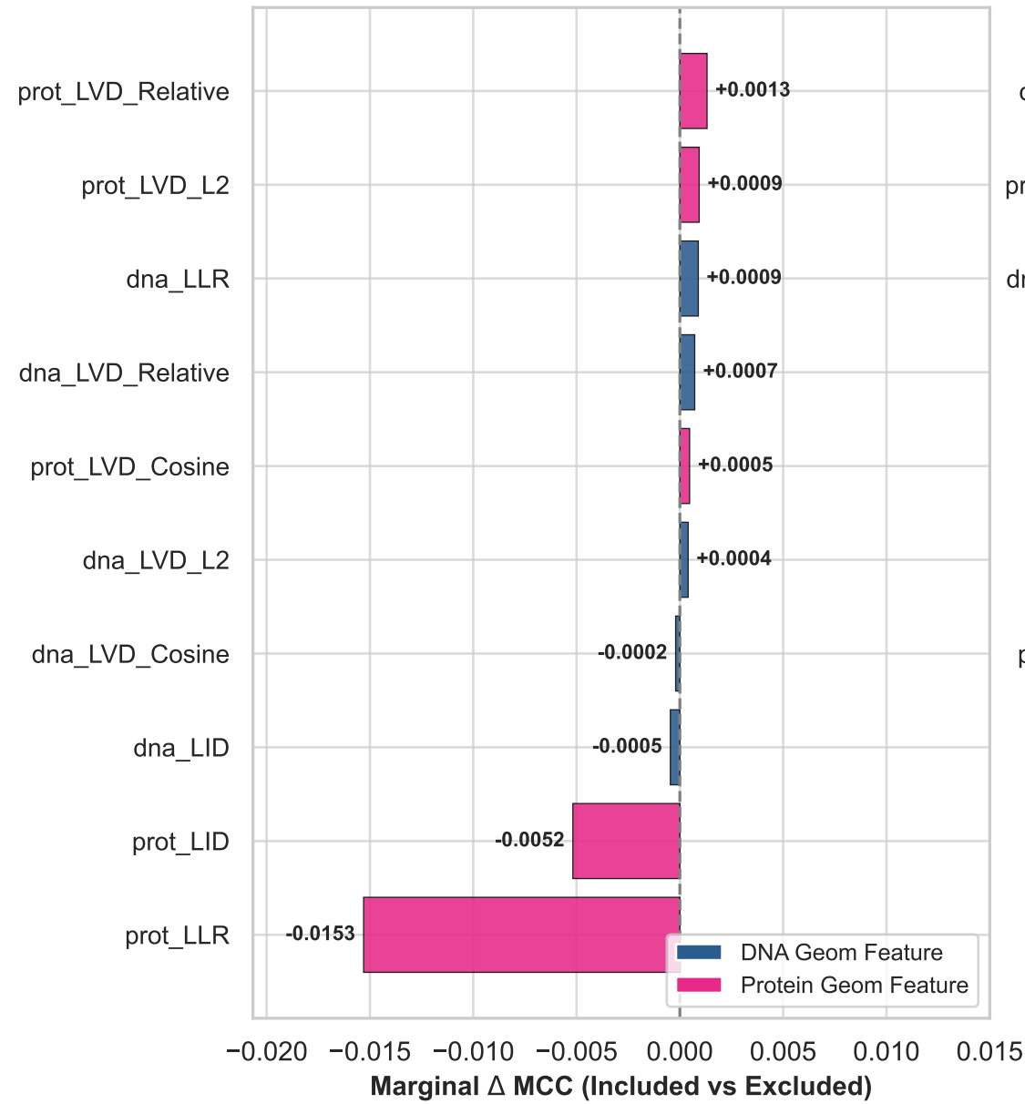
(A) Marginal Contribution of Geom Features (ClinVarHQ Benchmark)
