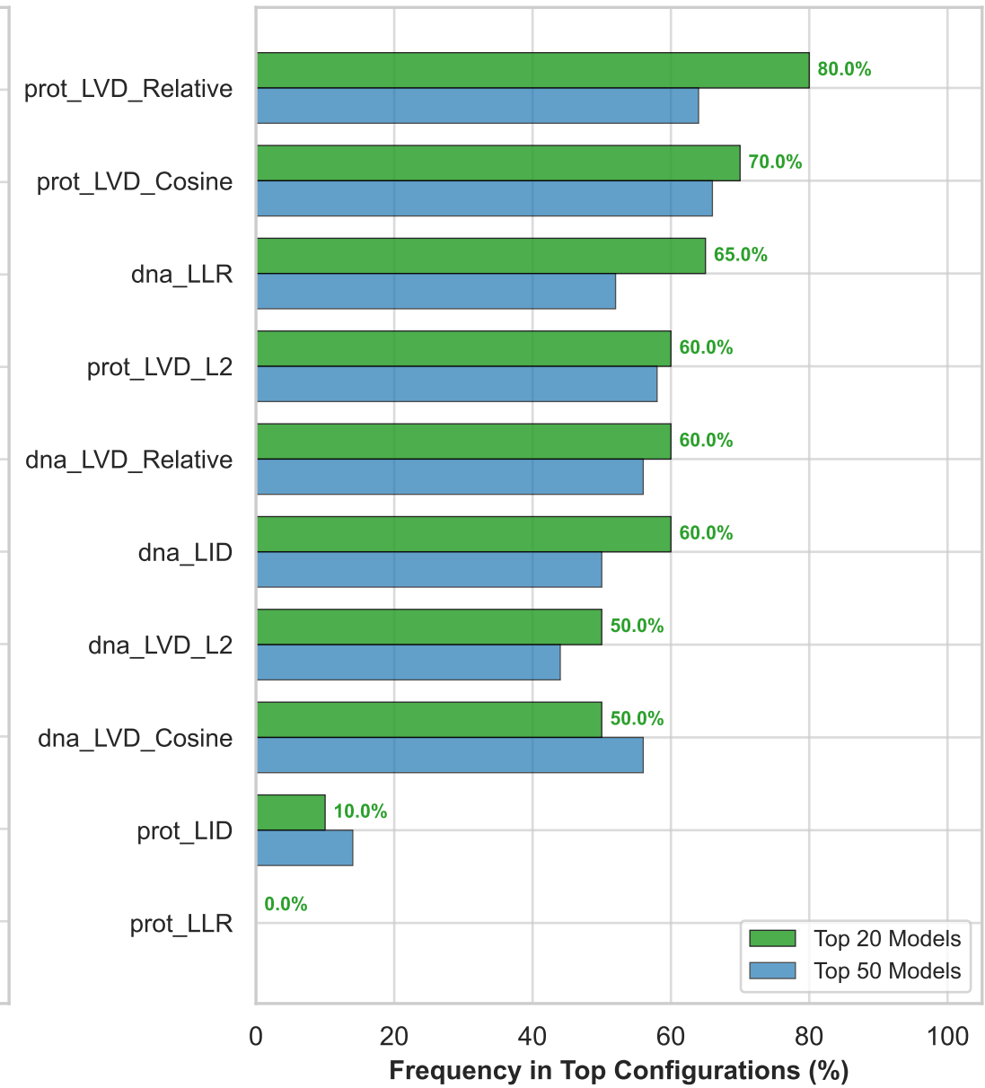
(C) Feature Selection Frequency (ClinVarHQ Benchmark)
