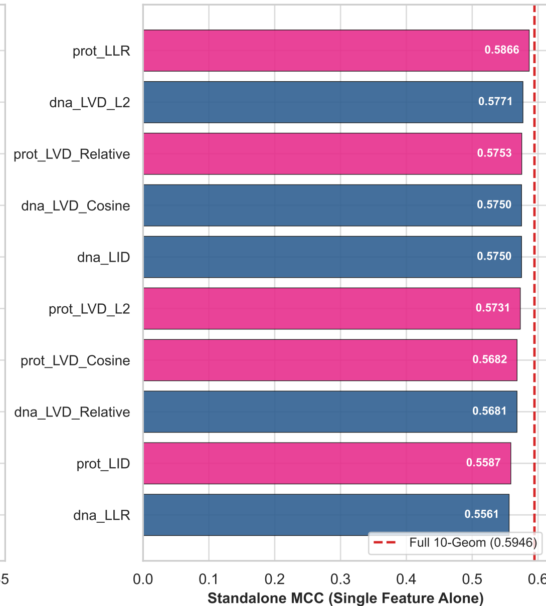
(B) Standalone Feature Performance (ProteinGym Benchmark)
