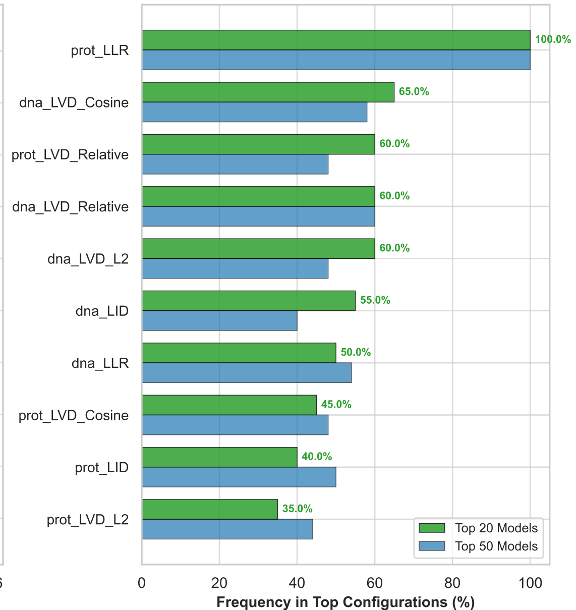
(C) Feature Selection Frequency (ProteinGym Benchmark)
