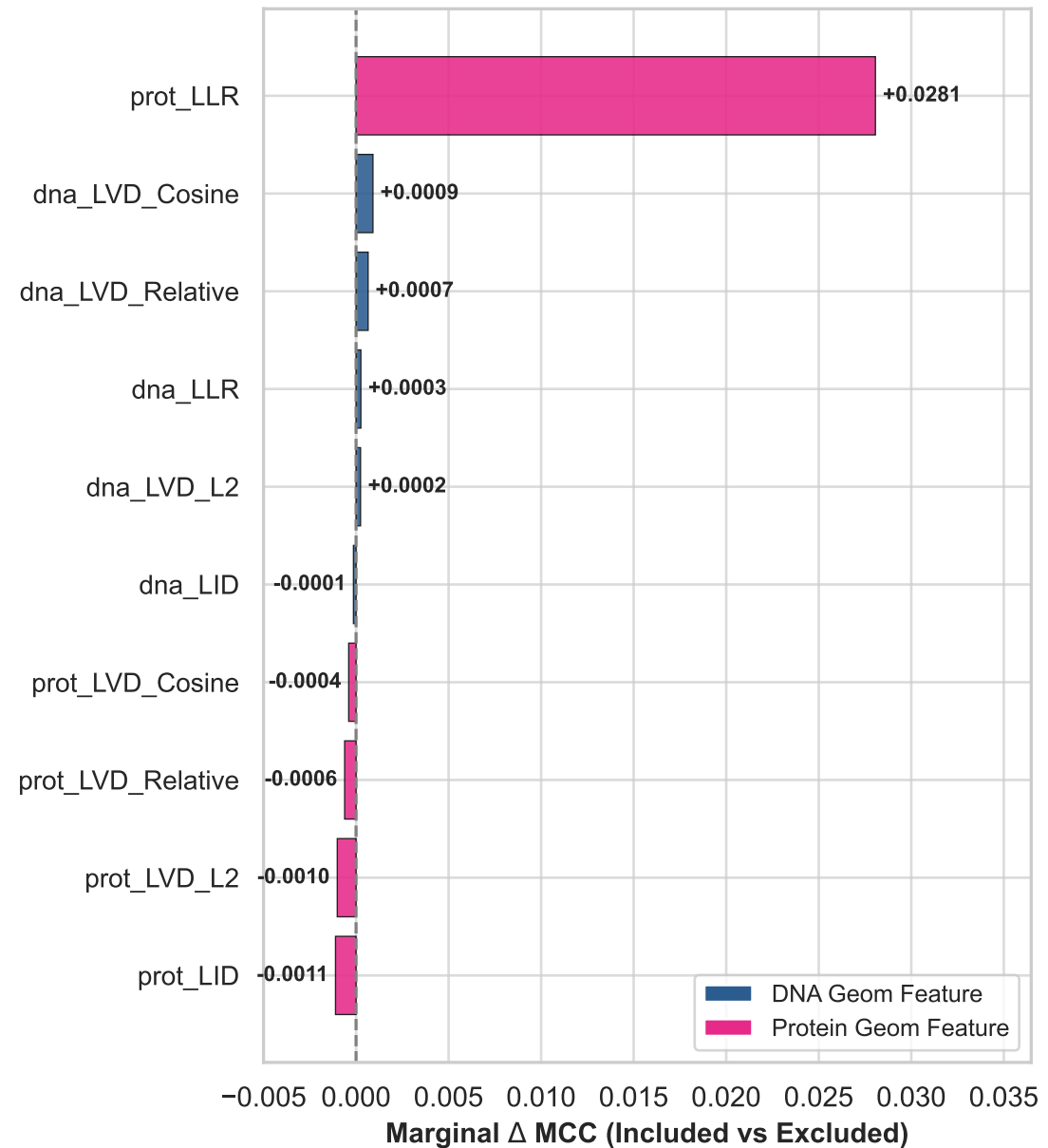
(A) Marginal Contribution of Geom Features (ProteinGym Benchmark)
