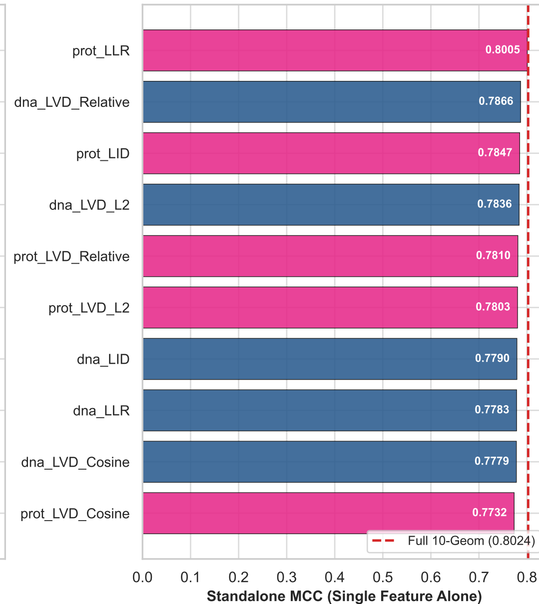
(B) Standalone Feature Performance (Test Benchmark)
