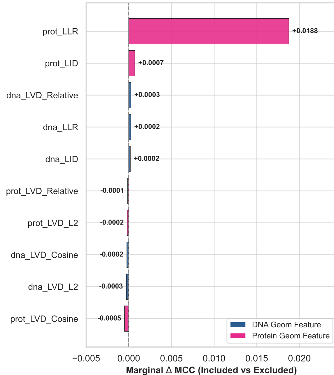
(A) Marginal Contribution of Geom Features (Test Benchmark)
