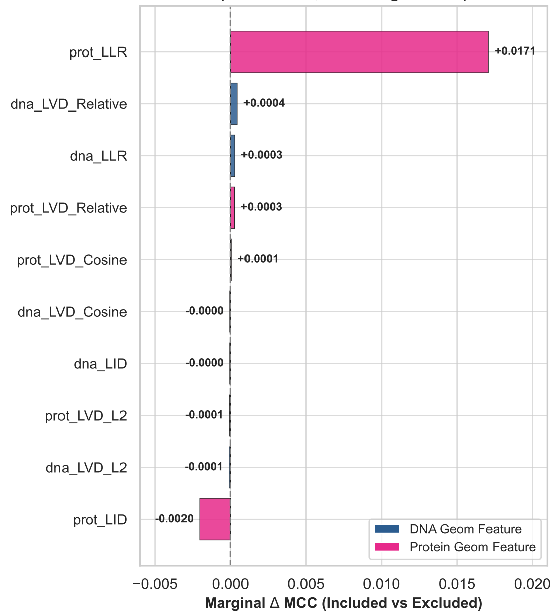
(A) Marginal Contribution of Geom Features (Across all 1,023 configurations)
