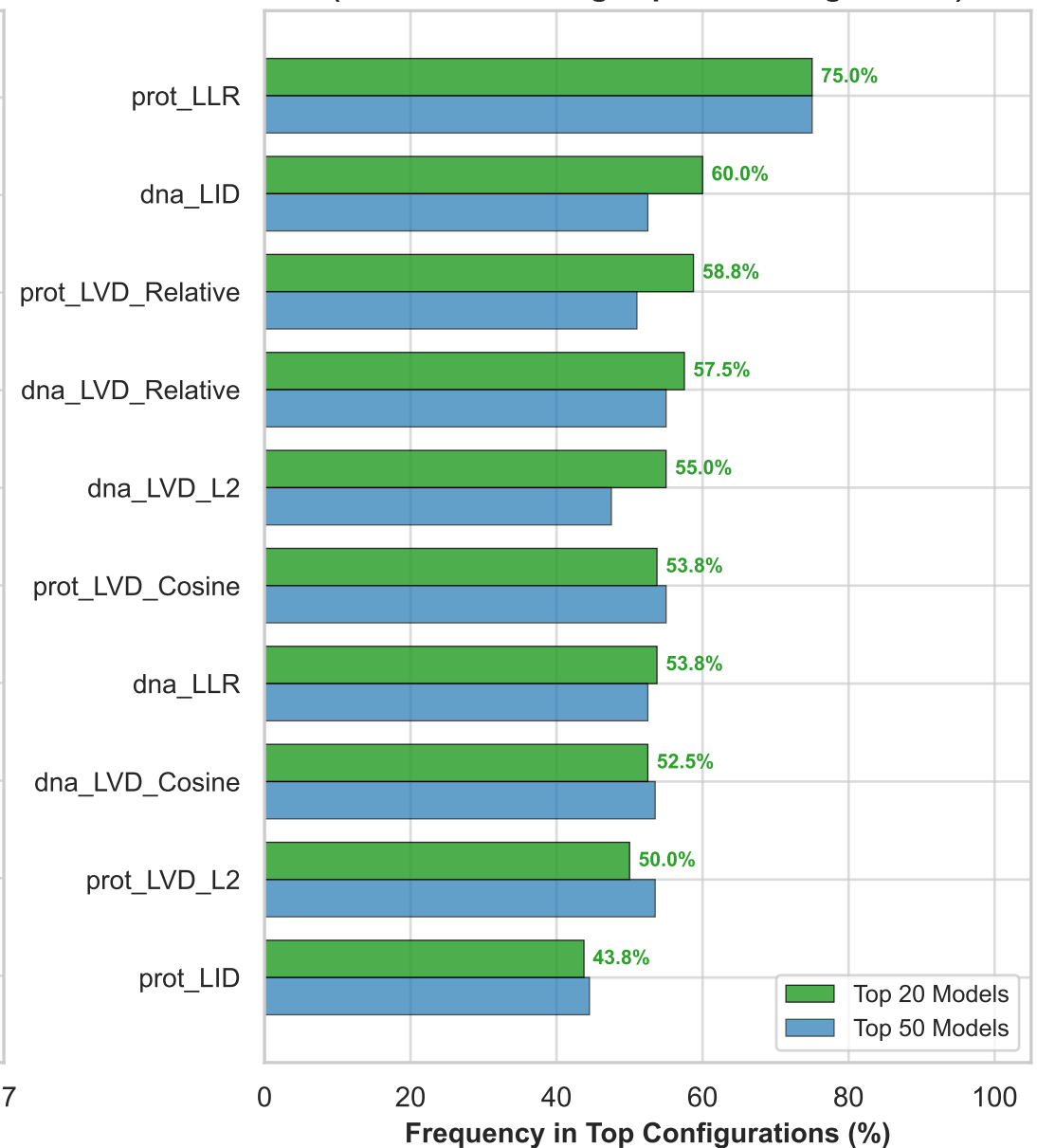
(C) Geometric Feature Selection Frequency (Prevalence among Top-Performing Models)
