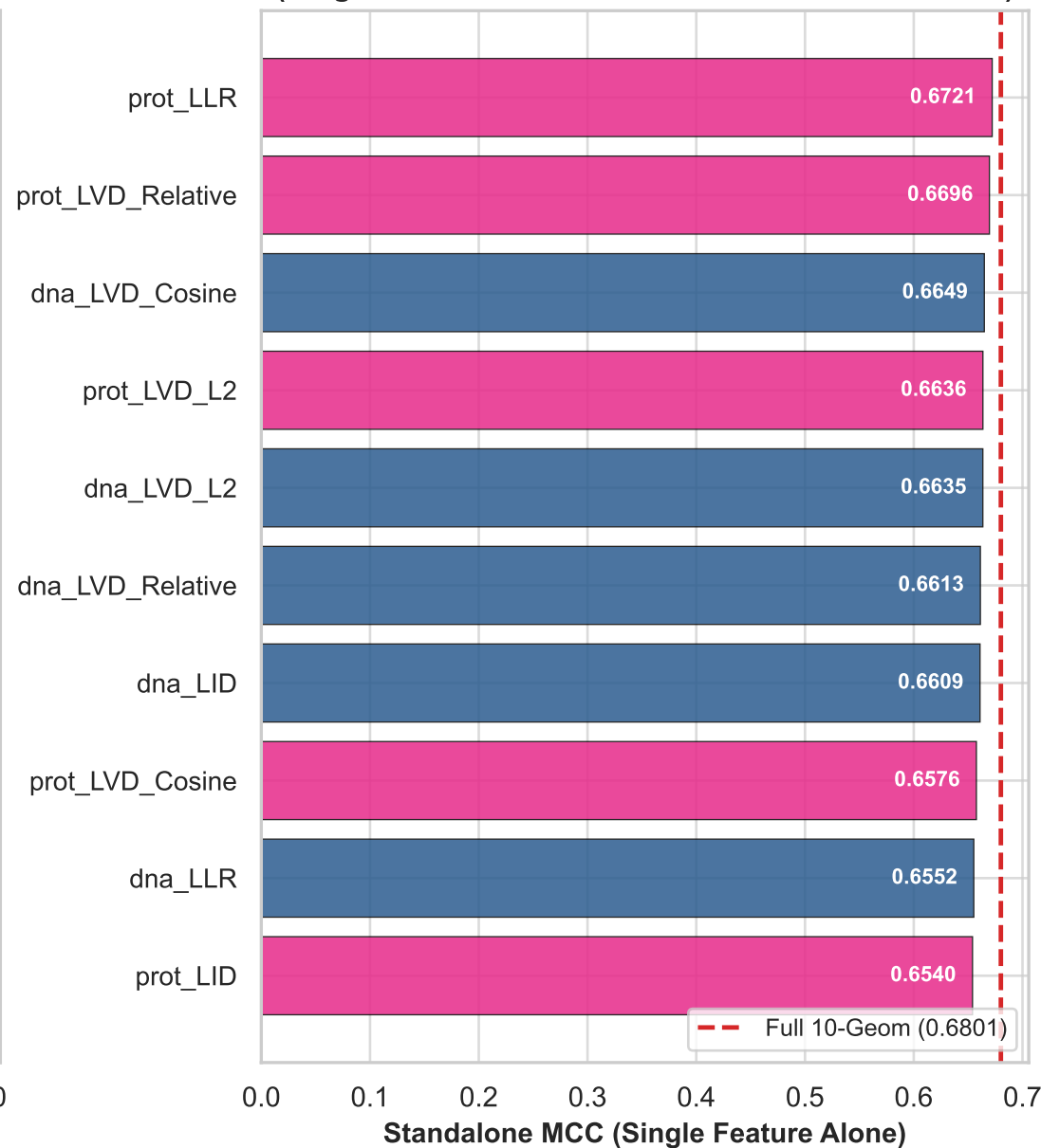
(B) Standalone Feature Performance (Single Feature Alone vs Full 10-Feature Ensemble)
